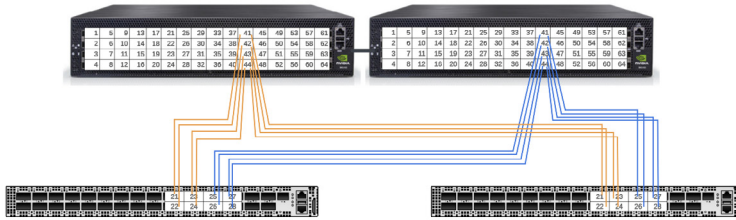
FIGURE 4 Example of aggregate connection uplinks from XFMs to the NVIDIA DGX GB200 SuperPOD SN5600 storage fabric
