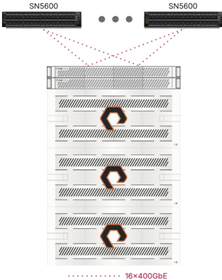
FIGURE 2 NVIDIA DGX GB200 SuperPOD storage fabric network integration
