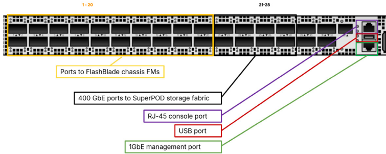
FIGURE 3 XFM port map
