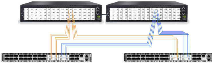
FIGURE 4 Example of aggregate connection uplinks from XFMs to the NVIDIA DGX GB300 SuperPOD SN5600 storage fabric
