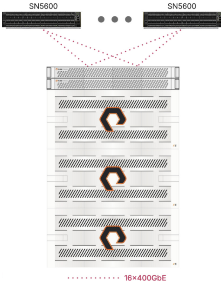
FIGURE 2 NVIDIA DGX GB300 SuperPOD storage fabric network integration
