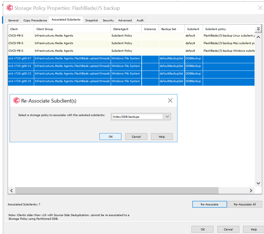
Figure 14. Reassociating subclients
