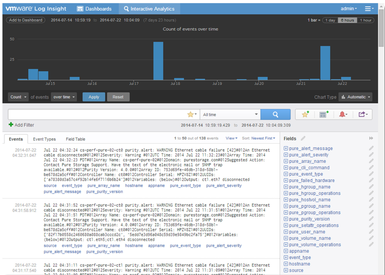
Figure 12. Pure Storage Extracted Fields
