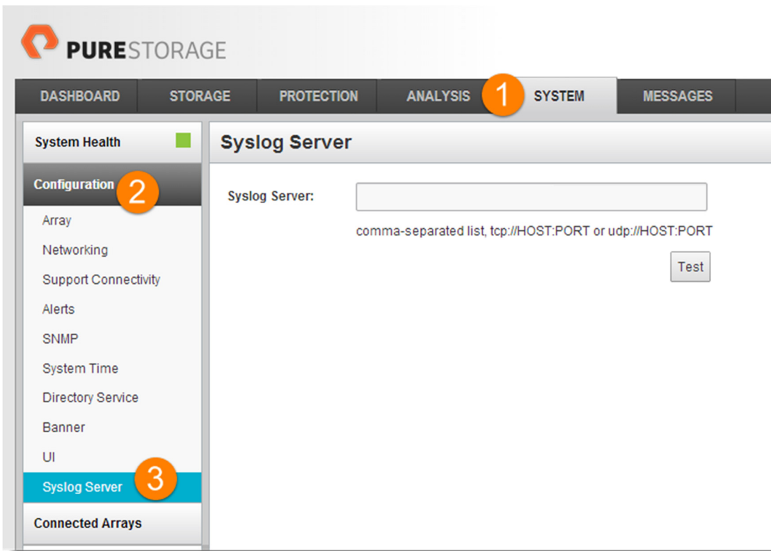
Figure 6. Locating the Syslog Server target host entry
